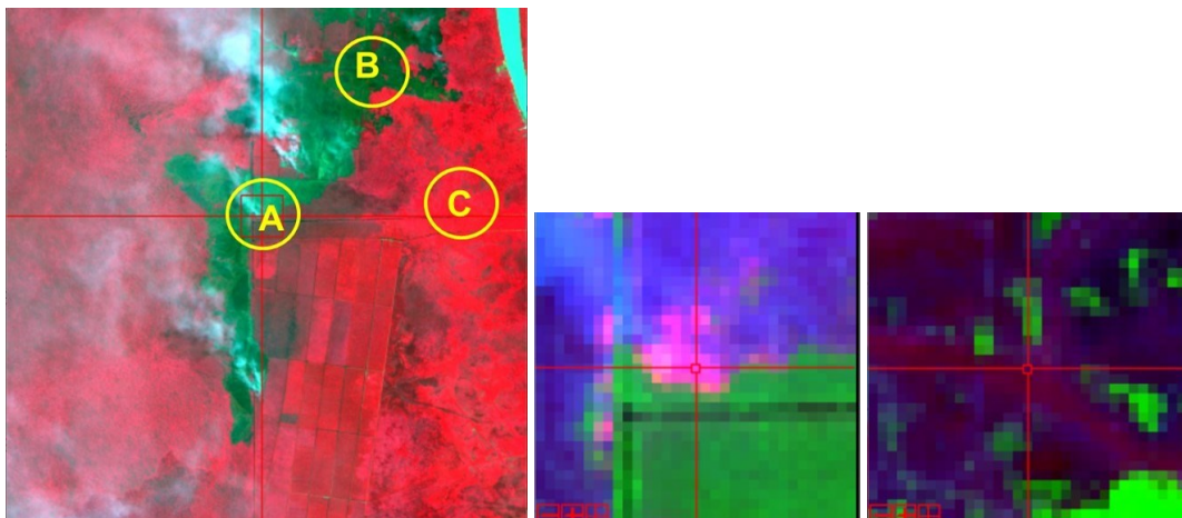
Figure 3. Sapling points for testing of the temperature retrieval model. Left: False color image (RGB = 8,4,3) showing the locations of the 3 points labeled A, B and C. Middle: Zoom-in image (RGB=12,8,4) of Location A, active fire. Right: Zoom-in image (RGB=12,8,4) of Location B, recent burn scar.
