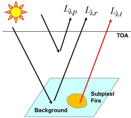
Figure 1. Components of the radiance detected at the top of the atmosphere from a sub-pixel fire
