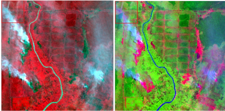
Figure 2. A subsene of a Sentinel-2A image showing smoke plumes of active fires and burn scars. False color display. Left: RGB = Bands 8,4,3. Right: RGB = Bands 12,8,4.
